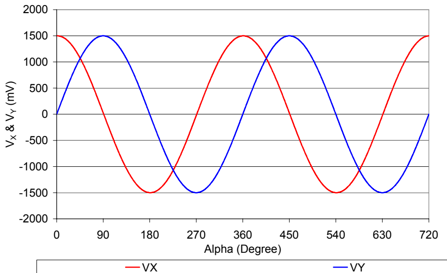
Figure 6 – Tria@is™ sensor front-end – Output signals – V_X \propto B_X \propto \cos(\alpha) & V_Y \propto B_Y \propto \sin(\alpha)
