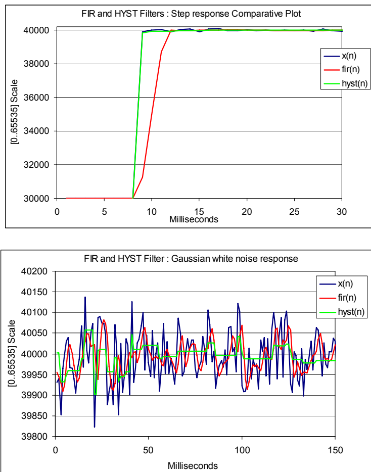
Figure 10 - Step Response and Noise Response for FIR (No 3) and FHYST=10
